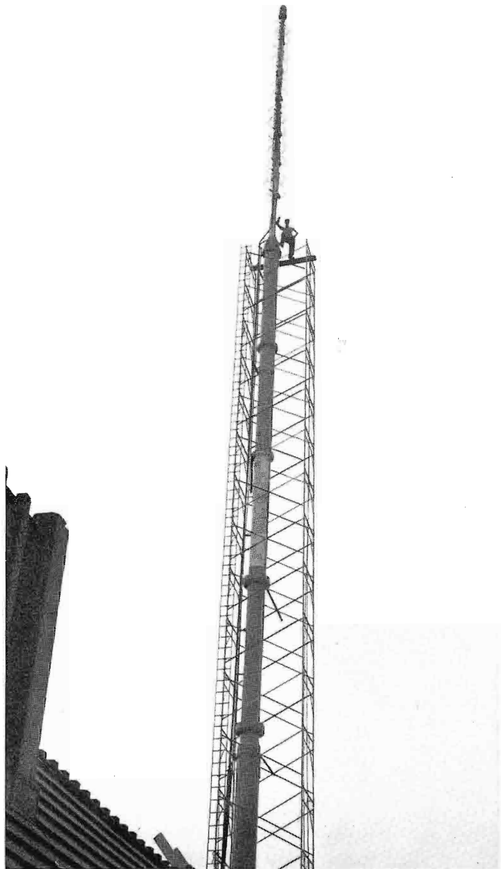
FIG. 25 (above). The Pylon sections were brought up one at a time. As each one was brought up it was stacked on top. Finally the Superturnstile was brought up (in one piece) and placed on top.
