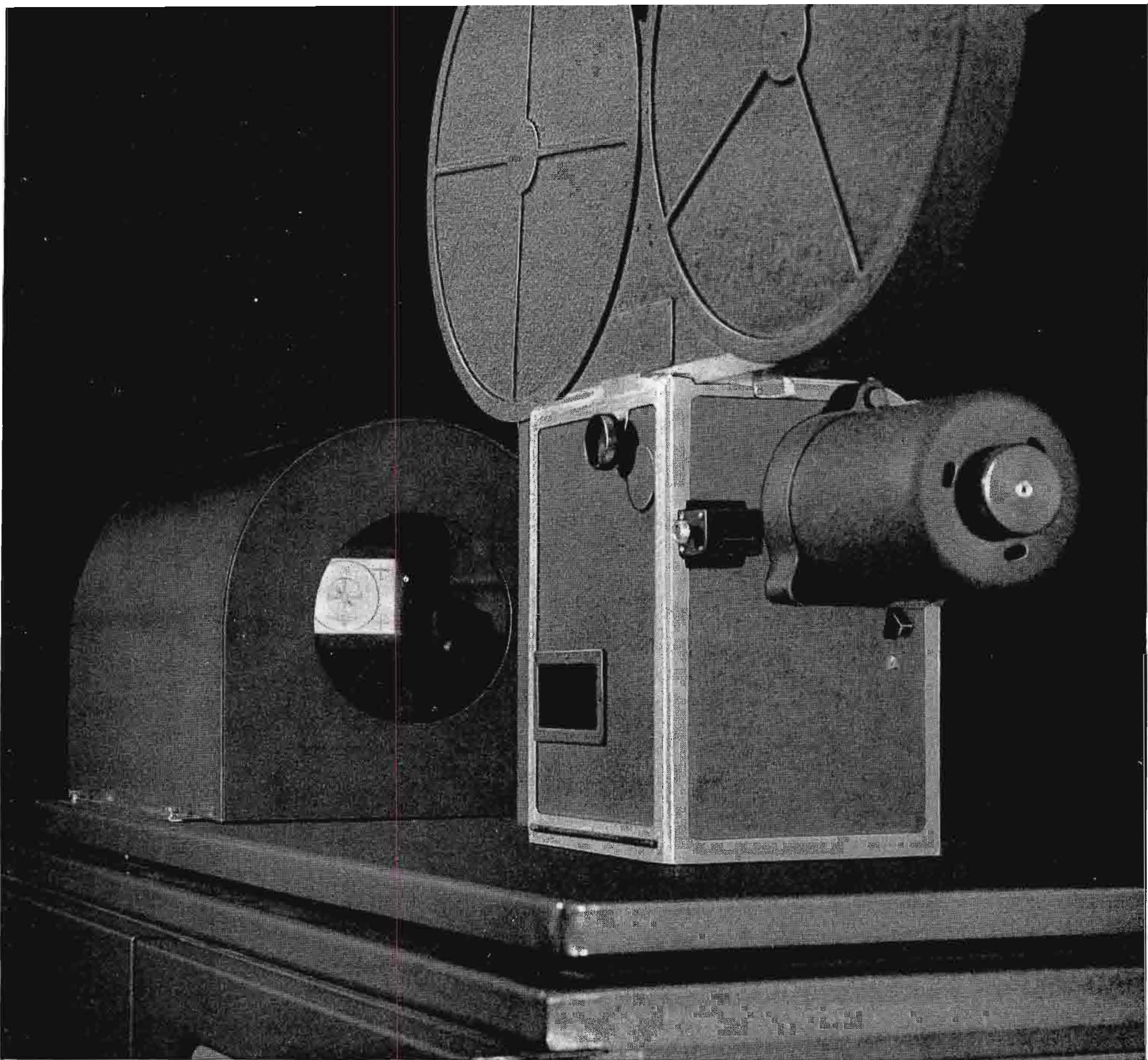
FIG. 6. The photo above shows a closeup of the RCA 16mm television camera which accommodates 1200 feet of film and which can be equipped for making simultaneous sound and film recordings. Either a 16mm or 35mm motion picture camera can be used to photograph the images appearing on the face of the projection type kinescope.
