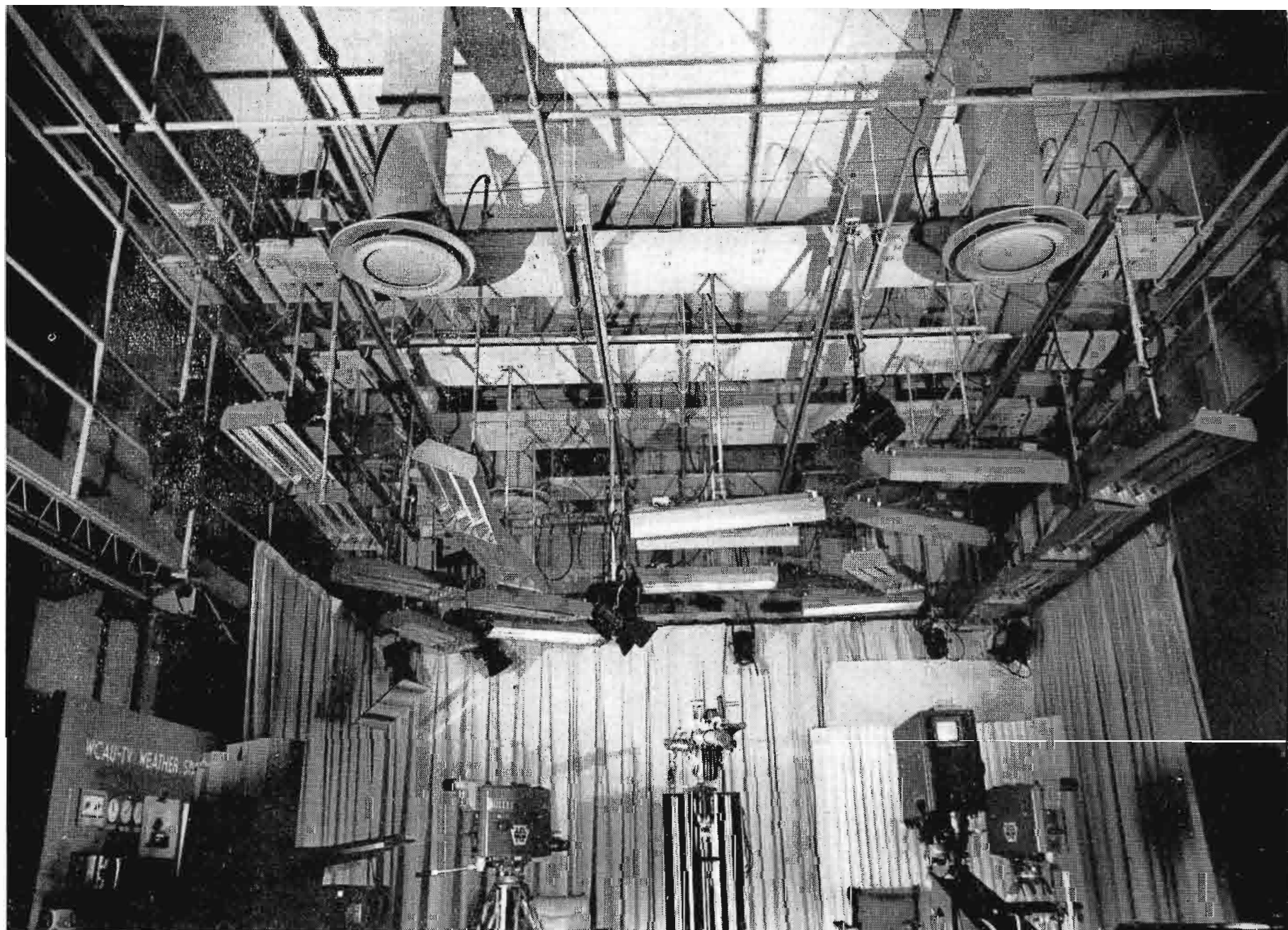
FIG. 21. Foundation lighting in WCAU-TV studios is obtained with specially designed fluorescent fixtures each of which contains three 40-watt 3500° standard fluorescent lamps. All fixtures can be rotated in any direction and adjusted as to height.
