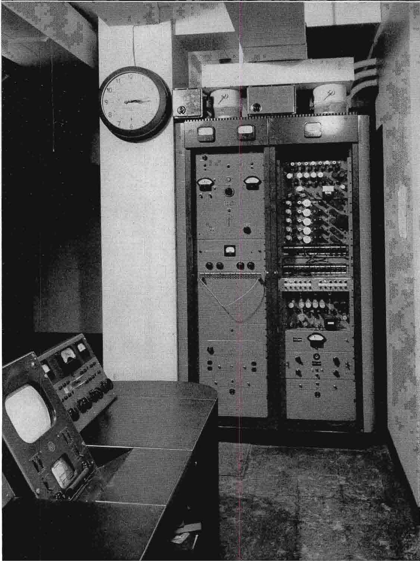
FIG. 19 (above). The view above shows the FM end of the transmitter control room (see floor plan, Fig. 8). The RCA BTF-10B FM Transmitter is at the right. At the left are racks containing audio and monitoring facilities, power supplies, etc. Turntable used for FM fill-ins and for testing is in the center. In the foreground is a corner of the TV transmitter control console.
