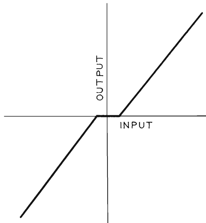
FIG. 8. BASIC OPERATION OF THE THRESHOLD NOISE SUPPRESSOR
