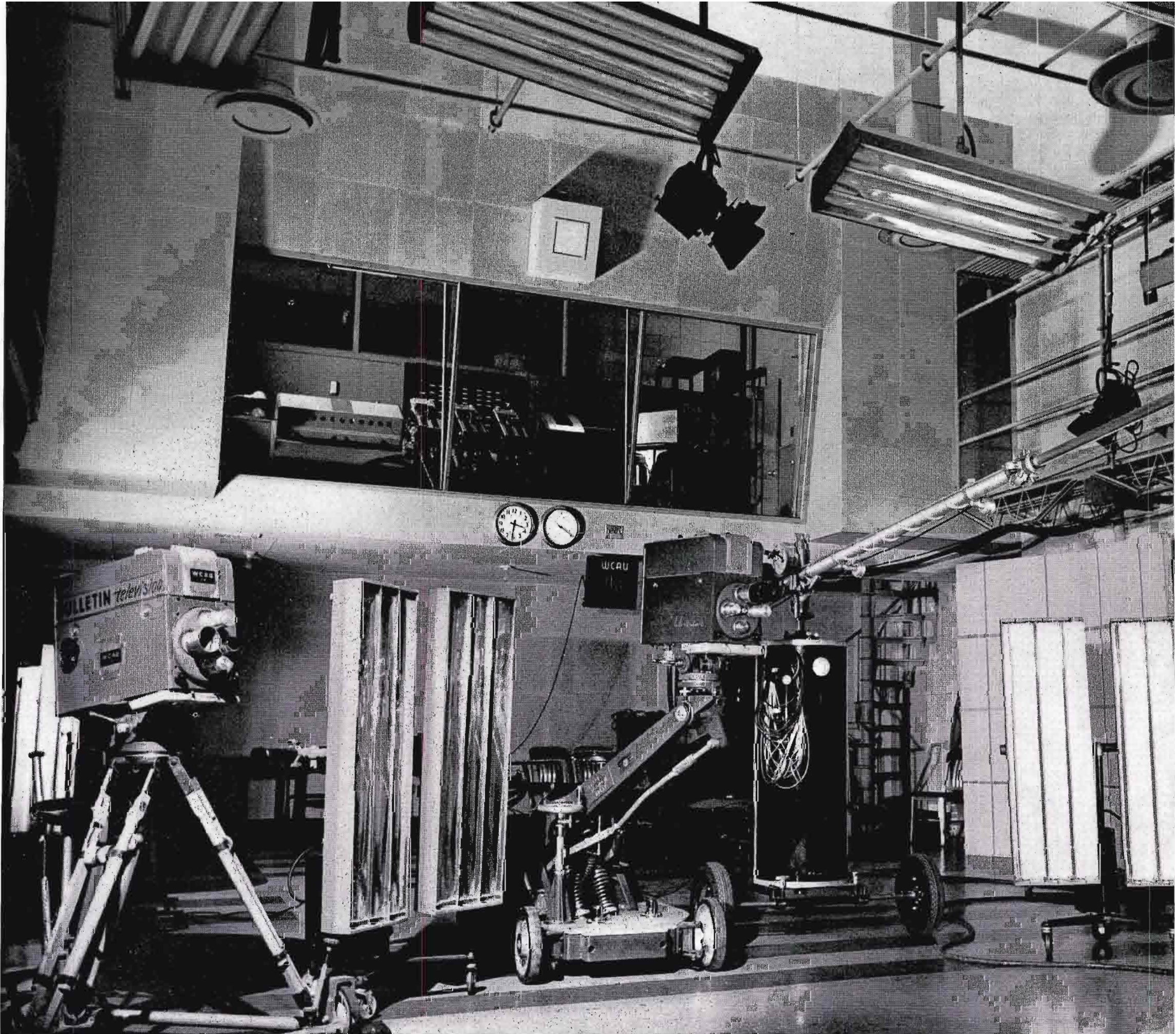
FIG. 5. This view of WCAU-TV's Studio A shows the elevated position of the control room. Space under the control room is available for camera maneuvering or for storage of scenery and props.
