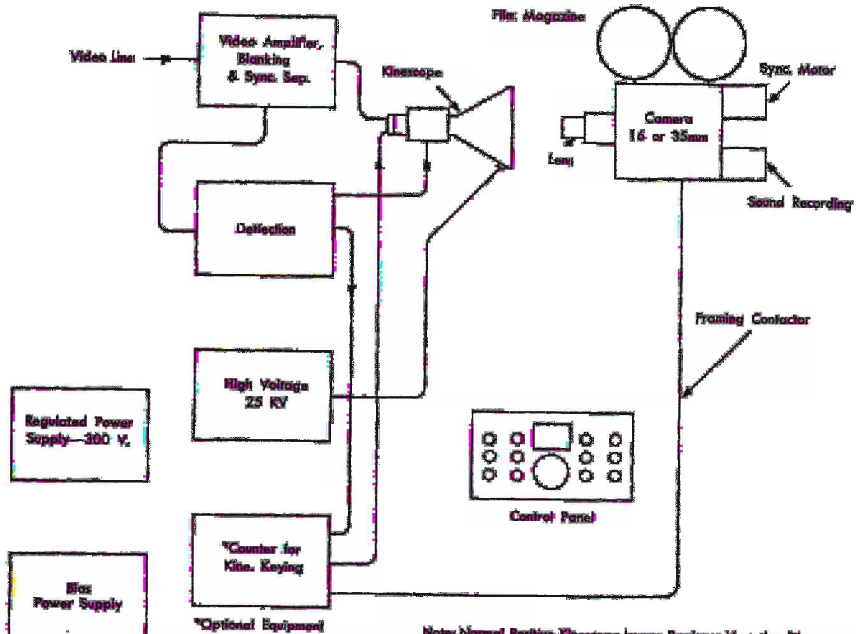
FIG. 3. This is a simplified block diagram of the RCA Kinescope Equipment which consists basically of a projection kinescope and its associated video amplifiers, deflection circuits, power supplies, and a special camera for making film recordings.
