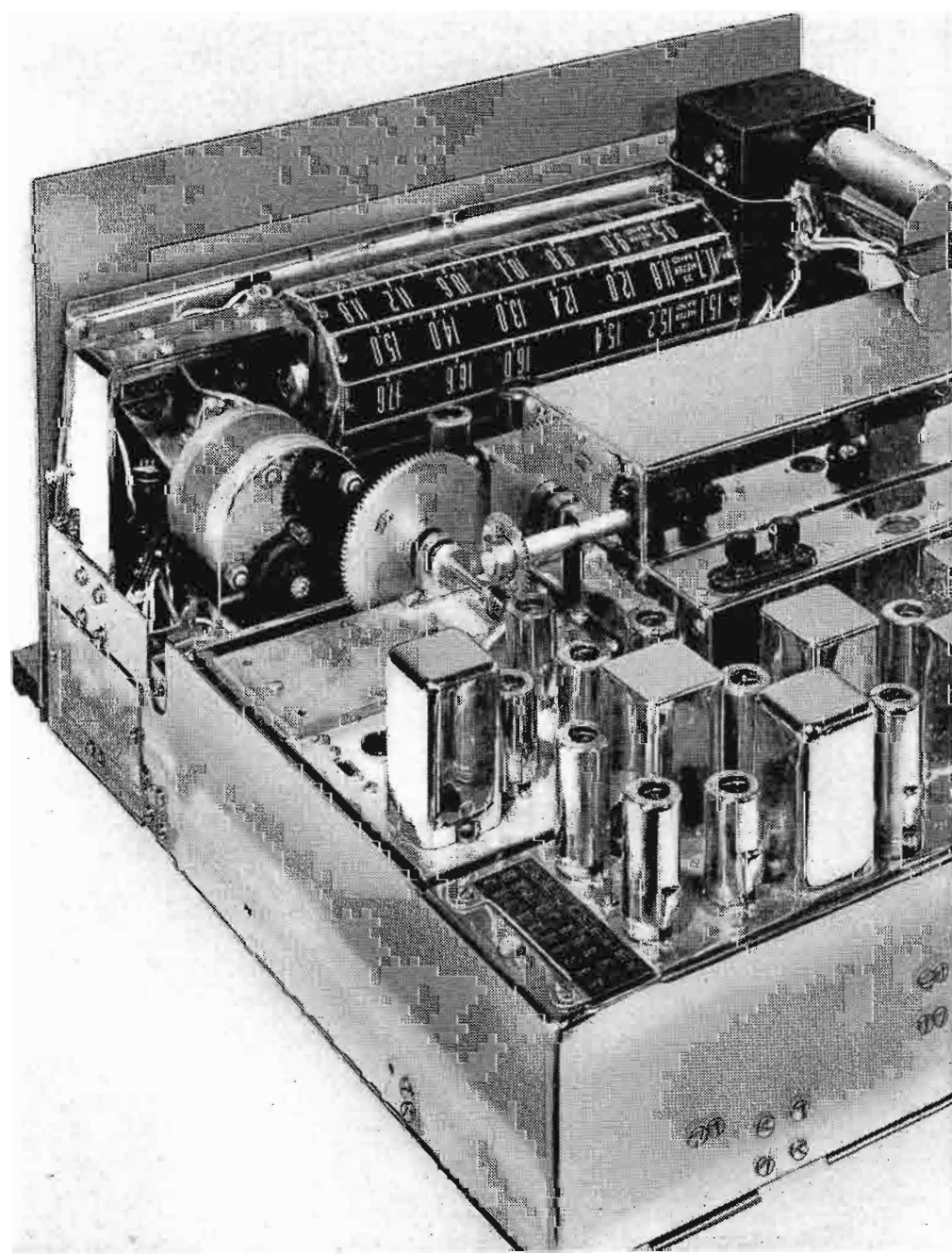
FIG. 3. The electrical components used in the Berkshire receivers are all of "broadcast quality." The r-f tuner which is shown below, for example, is copied from the famous AR-88 Receiver, RCA's outstanding commercial receiver.
