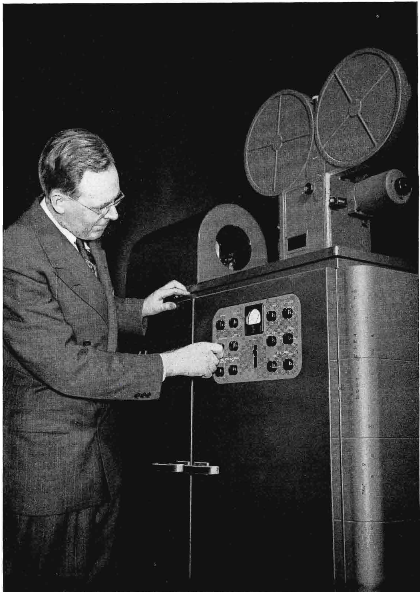
FIG. 2. R. V. Little, Jr., is shown adjusting the controls of the RCA Kinephoto Equipment. The unit shown is one of the earlier models. The control panels in newer units are equipped with built-in oscilloscopes which enable monitoring of the picture waveform.
