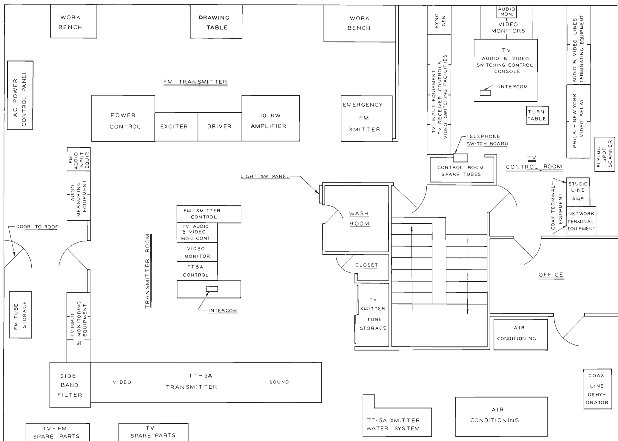
FIG. 25. Floor plan of WCAU-FM-TV transmitter installation showing arrangement of all major equipment items. Note provision of a separate TV Control Room containing terminal equipment as well as switching and monitoring equipment.
