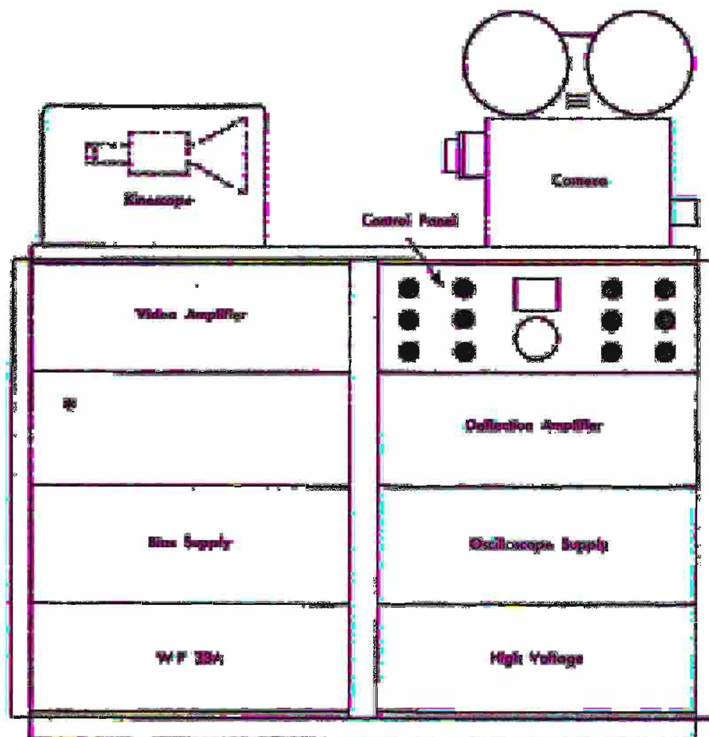
FIG. 4. This line drawing of the RCA unit shows the layout of the various components which are mounted in the double cabinet racks. An electronic exposure control unit is supplied as optional equipment.
