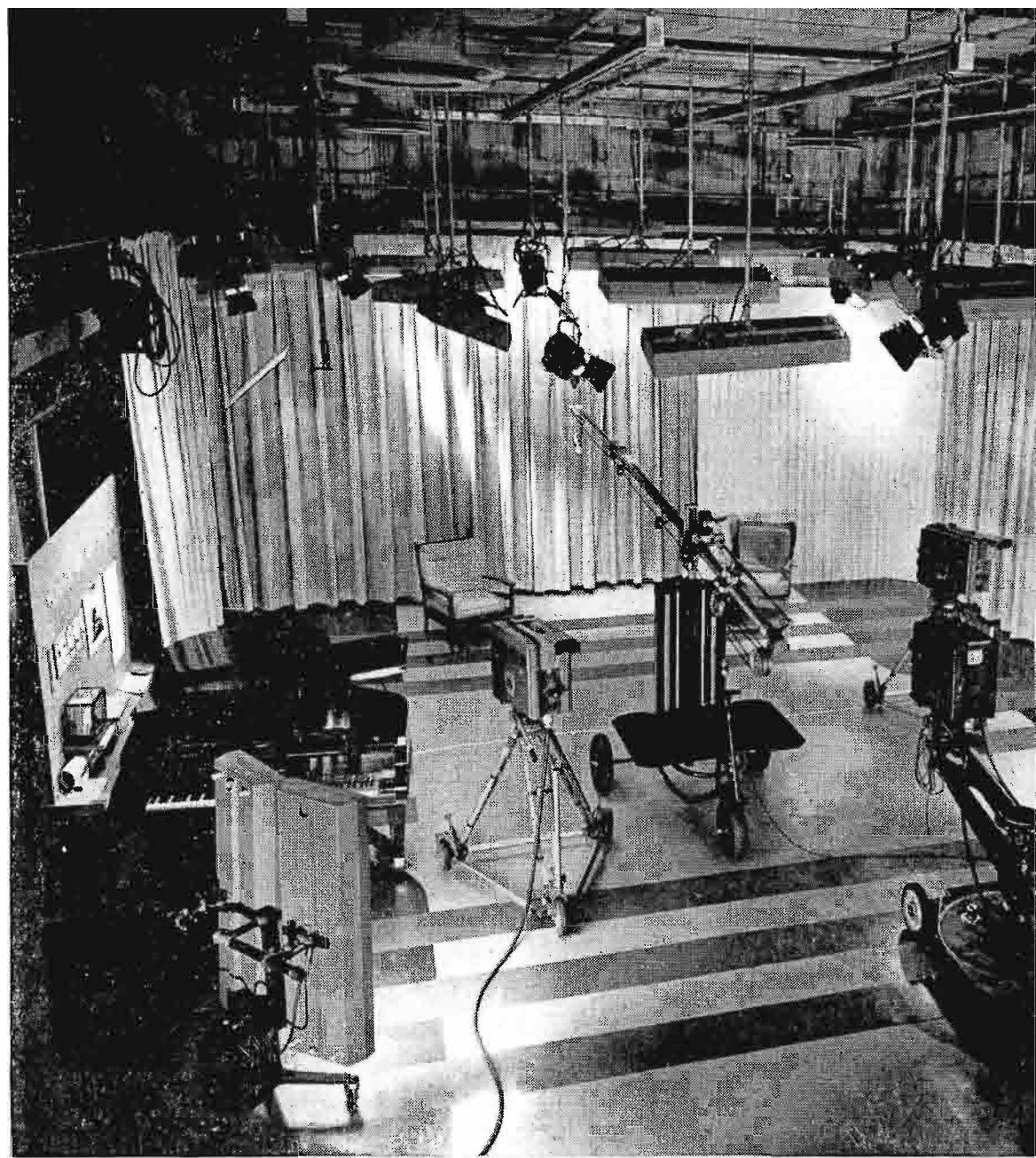
FIG. 20. Front lighting in WCAU-TV studios is supplied by adjustable fluorescent units similar to those mounted overhead.
