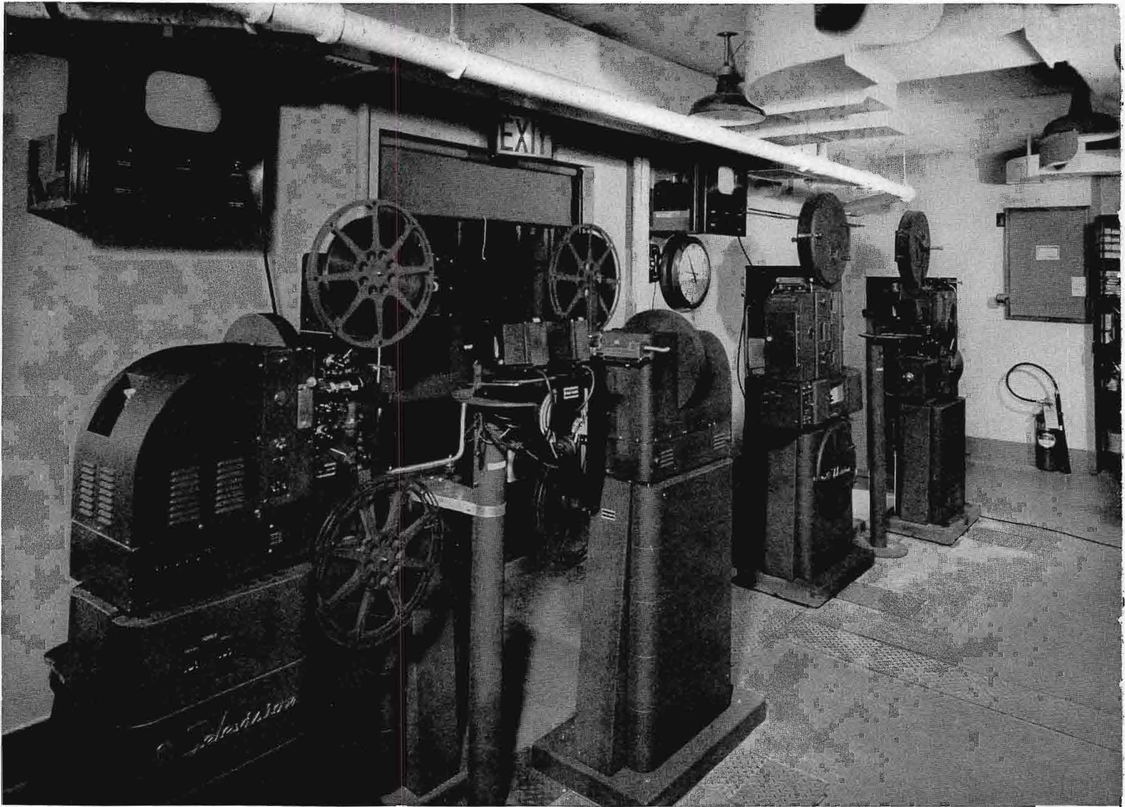
FIG. 16. This is WENR-TV's Film Projection Room. In the foreground are two RCA TP-16A (16mm) Projectors. Between them is a TP-9A Multiplexer and a TK-20A Film Camera. Further back are two RCA TP-35A (35mm) Projectors. Between them is a TP-9A Multiplexer and a TK-20A Film Camera. On the wall above each projector grouping is a monitor which allows the projectionist to see the picture transmitted.
