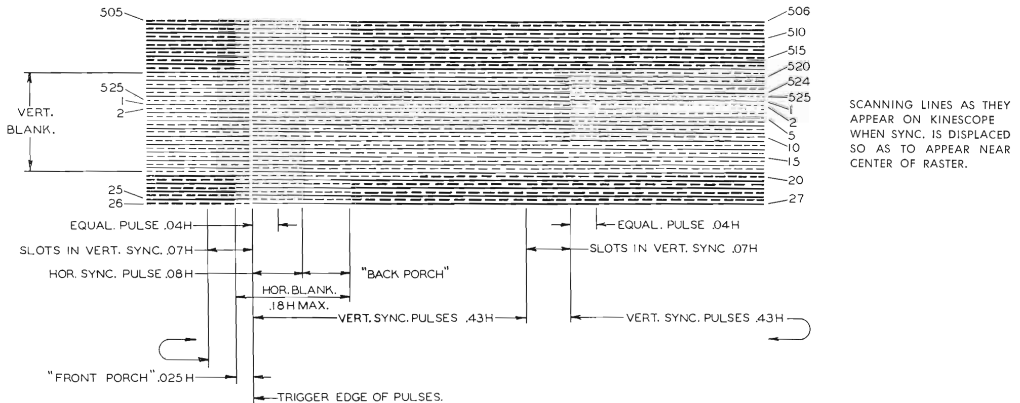
FIG. 9. A portion of the scanning lines appearing on a kinescope as a result of the application of a television signal composed of RMA sync. and blanking pulses. The group of lines shown are those occurring in the neighborhood of the vertical retrace period, including a few before and a few after the vertical blanking pulse.
