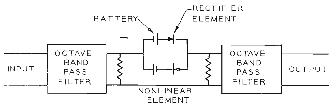
FIG. 8. BASIC OPERATION OF THE THRESHOLD NOISE SUPPRESSOR
